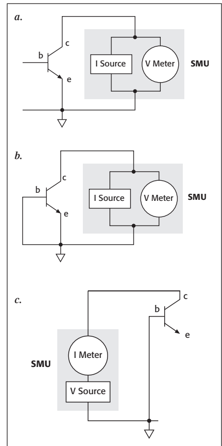
Figure 6: a: Collector-emitter breakdown with base open; b: Collector-emitter breakdown with base shorted; c: Collector cutoff current, ICBO , and collector-base breakdown voltage are measured with emitter open
